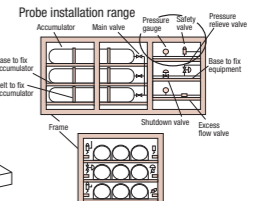
Fig.2 Example of Installation at Piping Module of Accumulators, etc.
