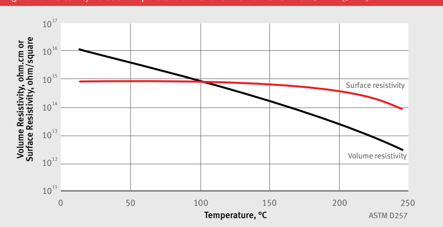
Figure 2. Resistivity versus Temperature of DuPont® Nomex® 818 — 0.13 mm (5 mil)
