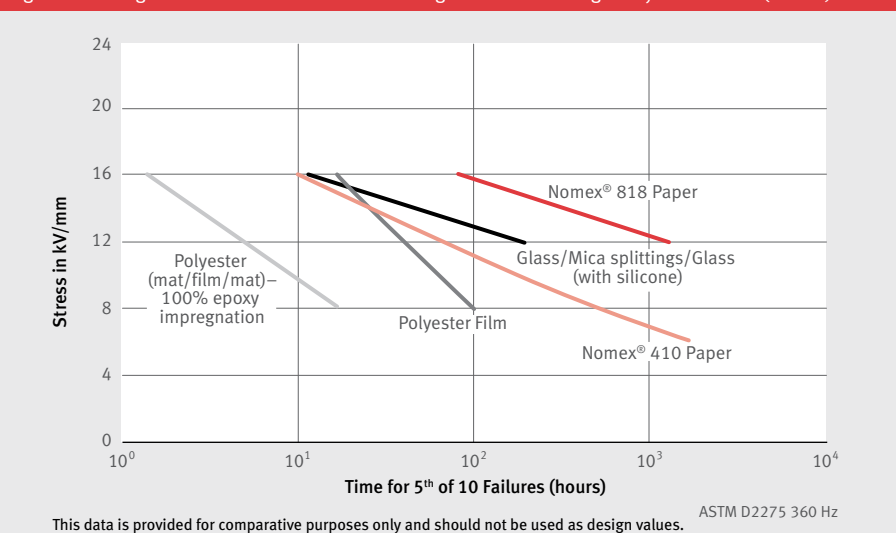
Figure 3. Voltage Endurance of Various Insulating Materials — Single-Layer 0.25 mm (10 mil)
